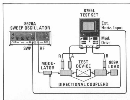
FIGURE 5. Setup for simultaneous swept measurement of insertion gain/loss and return loss.
