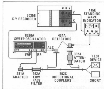
FIGURE 3. Typical waveguide reflectometer.
