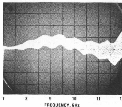
Figure 2. Multi-sweep slotted-line measurement. Vertical scale 0.5 dB/cm.
