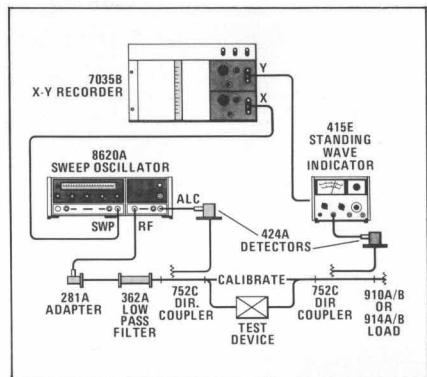
FIGURE 4. Swept attenuation system for measurements up to 30 dB.
